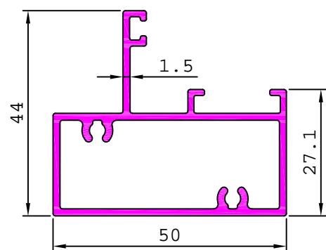
S5268 0.818 kg/m
