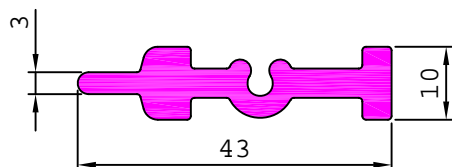
S5241 0.638 kg/m
