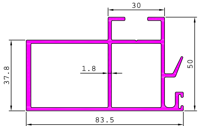
S5192 1.642 kg/m
