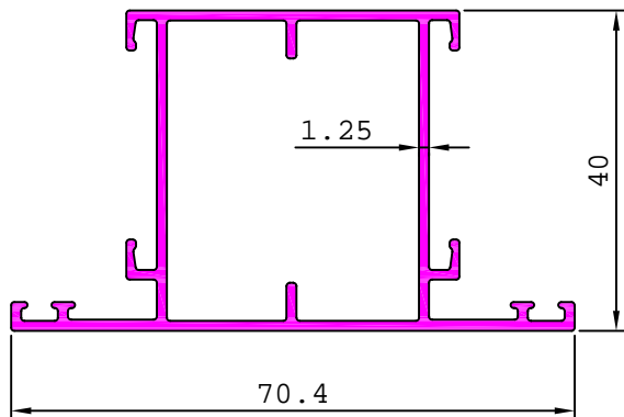
S5181 0.782 kg/m
