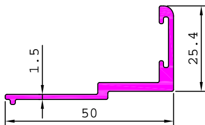
S5240 0.453 kg/m
