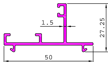
S5269 0.403 kg/m
