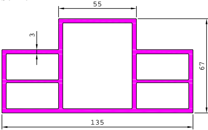
S6176 4.209 kg/m
