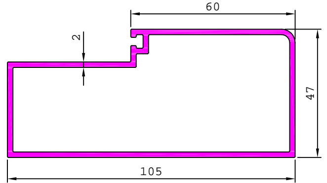
S6177 3.560 kg/m
