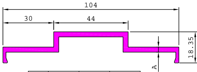
S5745 1.624 kg/m
